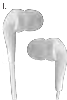
$5.90 iLive Earbuds • 10mm Driver • 3.9 ft Flat Cord • Impedance: 32 Ohms • Sensitivity: 102dB • Frequency Response: 20 - 20,000 Hz • Includes 2 Sets of Earpads • Shipping Weight: 1 oz. 7010-122 ..... Price $5.90
